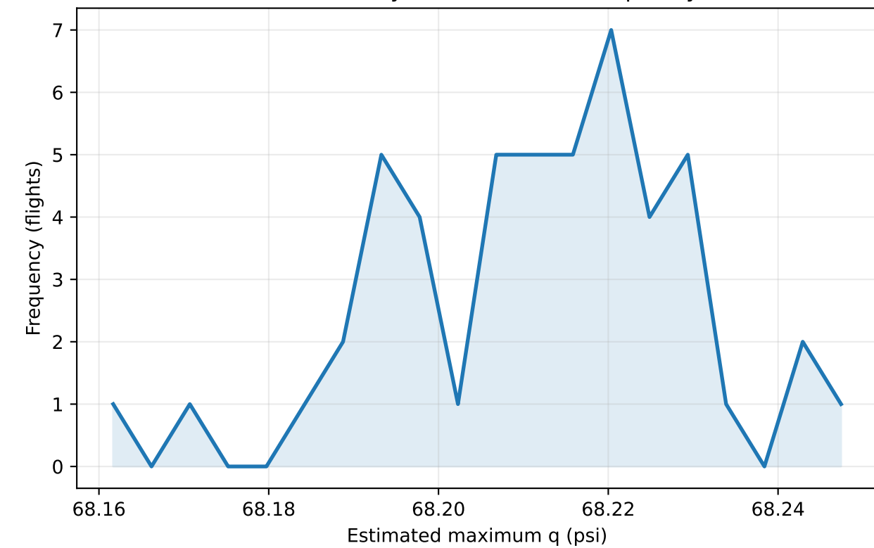
Maximum Dynamic Pressure Frequency
